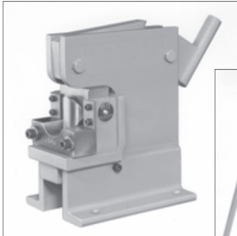
#1400 Hand Press with Housing & Assembly (sold separately)
