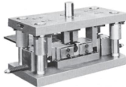
SPECIAL DOUBLE SIDE NOTCH DIE With double clamp-up action to notch two 1" long by ¼" wide windows in 1" O.D. x 20 Ga. tubing.
