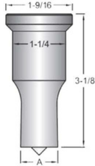
770 Punch
