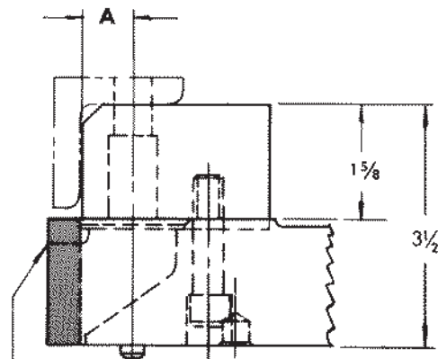
MACHINE FRONT FACE OF CASTING, IF NECESSARY, TO CLEAR WORK PIECE
